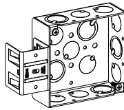
"MS" BRACKET Self-Gripping Metal Stud Bracket with Box Support Clip
